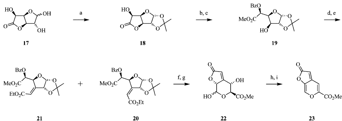
Scheme 5. (a) Me 2 CO, H 2 SO 4 ; (b) BzCl, C 5 H 5 N; (c) Et 3 N, MeOH, 79% from 18 ; (d) PDC, Ac 2 O, CH 2 Cl 2 ; (e) Ph 3 PCHCO 2 Et, CH 2 Cl 2 ( 21/20 , 1:99), 0.8% and 88% from 19 , respectively; (f) NaCN, MeOH; (g) CF 3 CO 2 H, H 2 O, 81% from 20 ; (h) Ac 2 O, C 5 H 5 N; (i) DBU, CH 2 Cl 2 , 68% from 22 .
