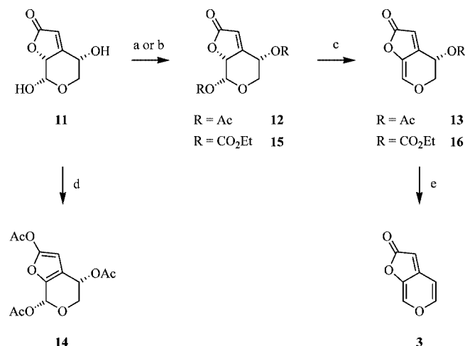
Scheme 4. (a) \text{Ac}_2\text{O} , \text{C}_5\text{H}_5\text{N} , 95%; (b) \text{EtOCOC}_2\text{H}_5 , \text{C}_5\text{H}_5\text{N} , 93%; (c) \text{Et}_3\text{N} , \text{CH}_2\text{Cl}_2 , 94% or 95%; (d) \text{Ac}_2\text{O} , \text{Et}_3\text{N} , \text{C}_5\text{H}_5\text{N} , 91%; (e) (\text{Ph}_3\text{P})_4\text{Pd} , THF, 84%.
